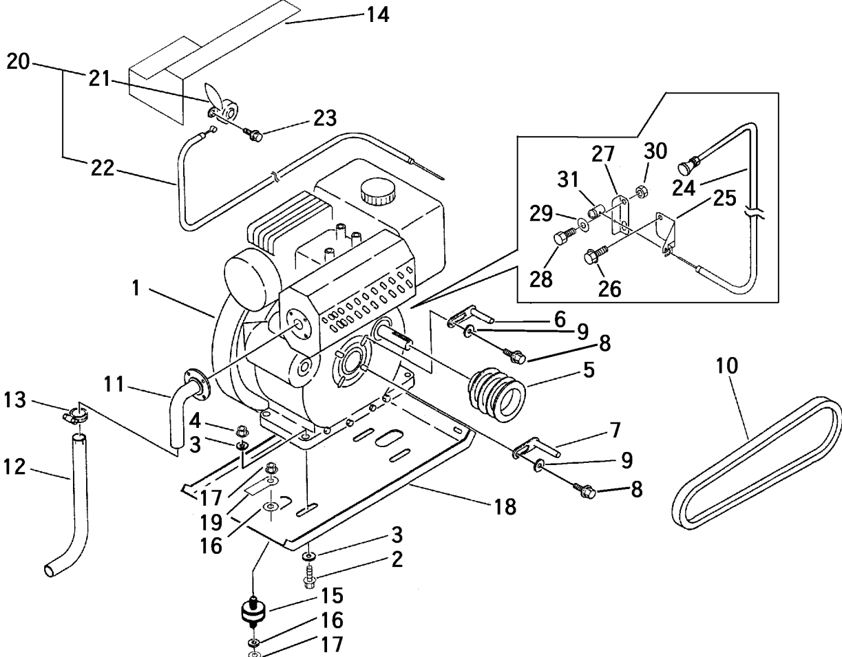
ENGINE & ENGINE CONTROL
